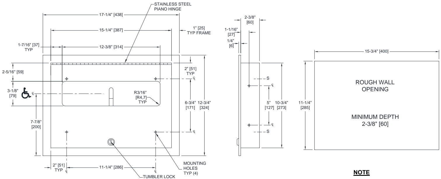
FRONT VIEW
